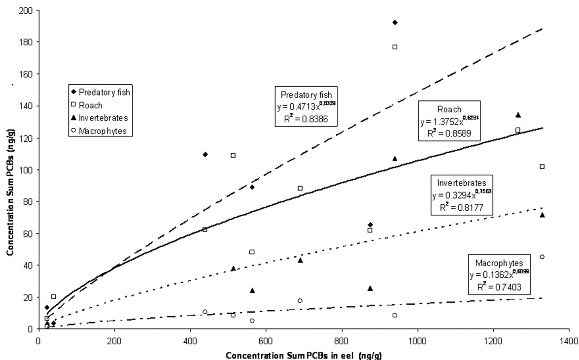
Fig. 7. – Correlation between the concentration of Sum PCBs measured simultaneously in predator fish species, roach, invertebrates and macrophytes, compared to the concentration of Sum PCBs in eel. Data acquired from sampling on five polluted water bodies in Flanders during spring and autumn 2001 (Weltens et al. 2002). Concentrations are expressed in ng/g wet weight of muscle tissue for fish and in ng/g total wet weight for invertebrates and macrophytes.
