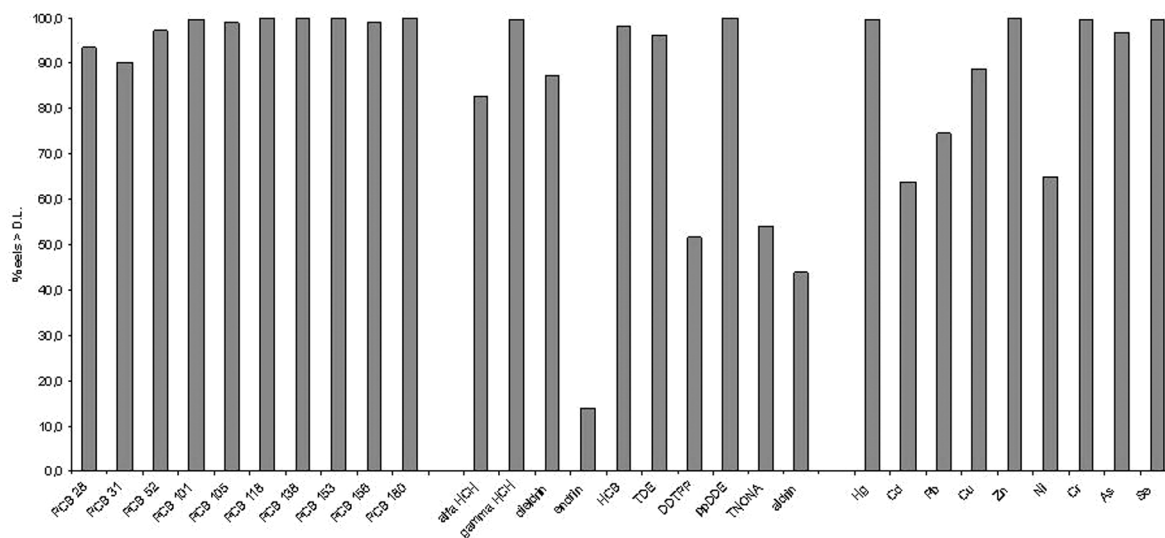
Fig. 2. – Percentage of individual yellow eel measurements above the detection limit for 10 PCB congeners and 10 organochlorine pesticides and 9 heavy metals in eels from Flanders collected in the period 1994-2005. N = 2528 for the PCBs, hexachlorocyclohexanes (HCHs), dieldrin, hexachlorobenzene (HCB), DDTs, trans-Nonachlor (TNONA) and endrin, N = 546 for aldrin, N = 2769 for Hg, Cd and Pb, N = 2117 for Cu, Zn, Ni and Cr and N = 1410 for As and Se (data from INBO Eel Pollution Monitoring Network). For an overview of the mean eel life history statistics (length, weight and lipid content) see Maes et al. (2007).
